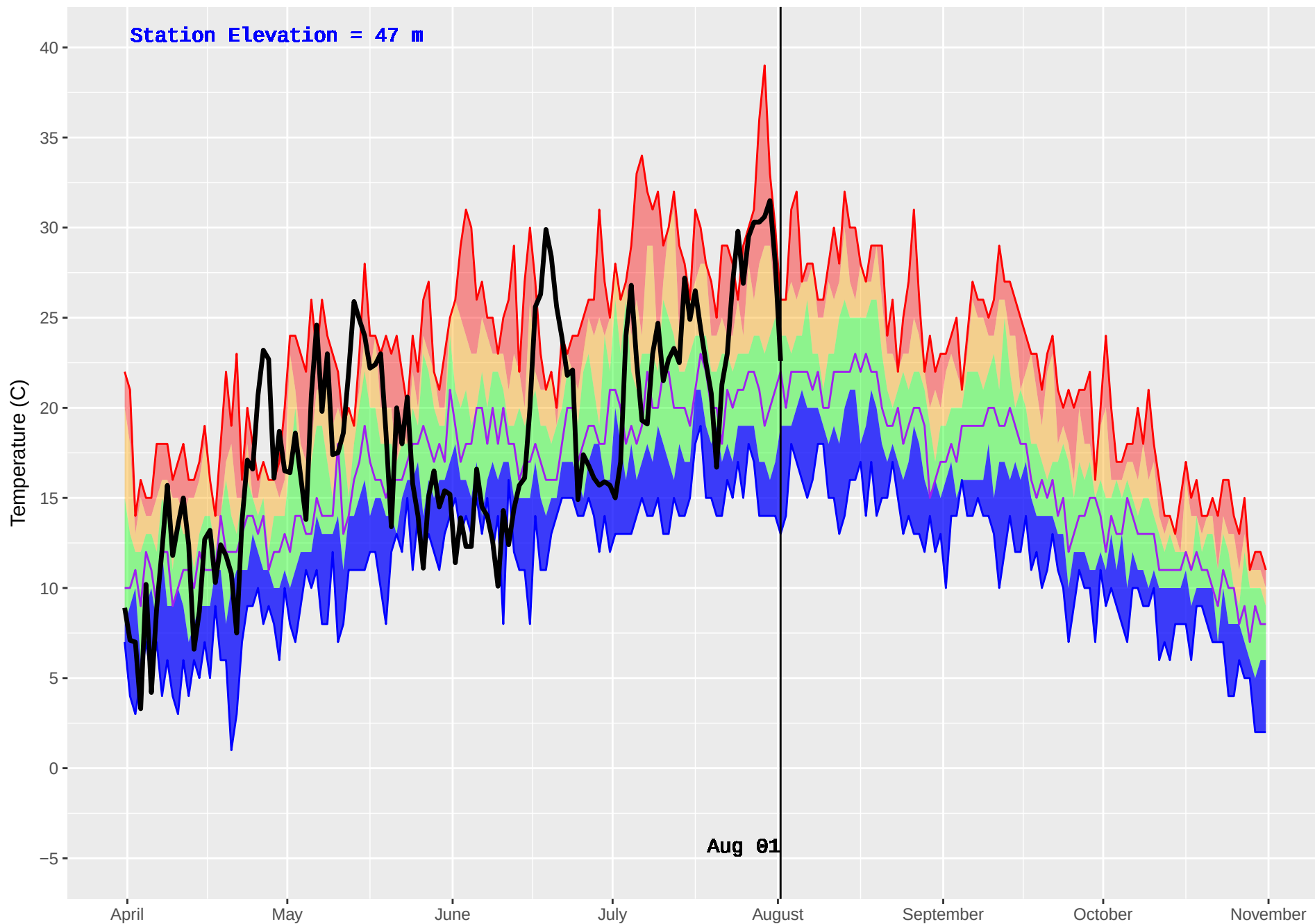
HAGENSBORG 2 (904) : Historical (2005–2016) and Current (2018) Daily Temperature
