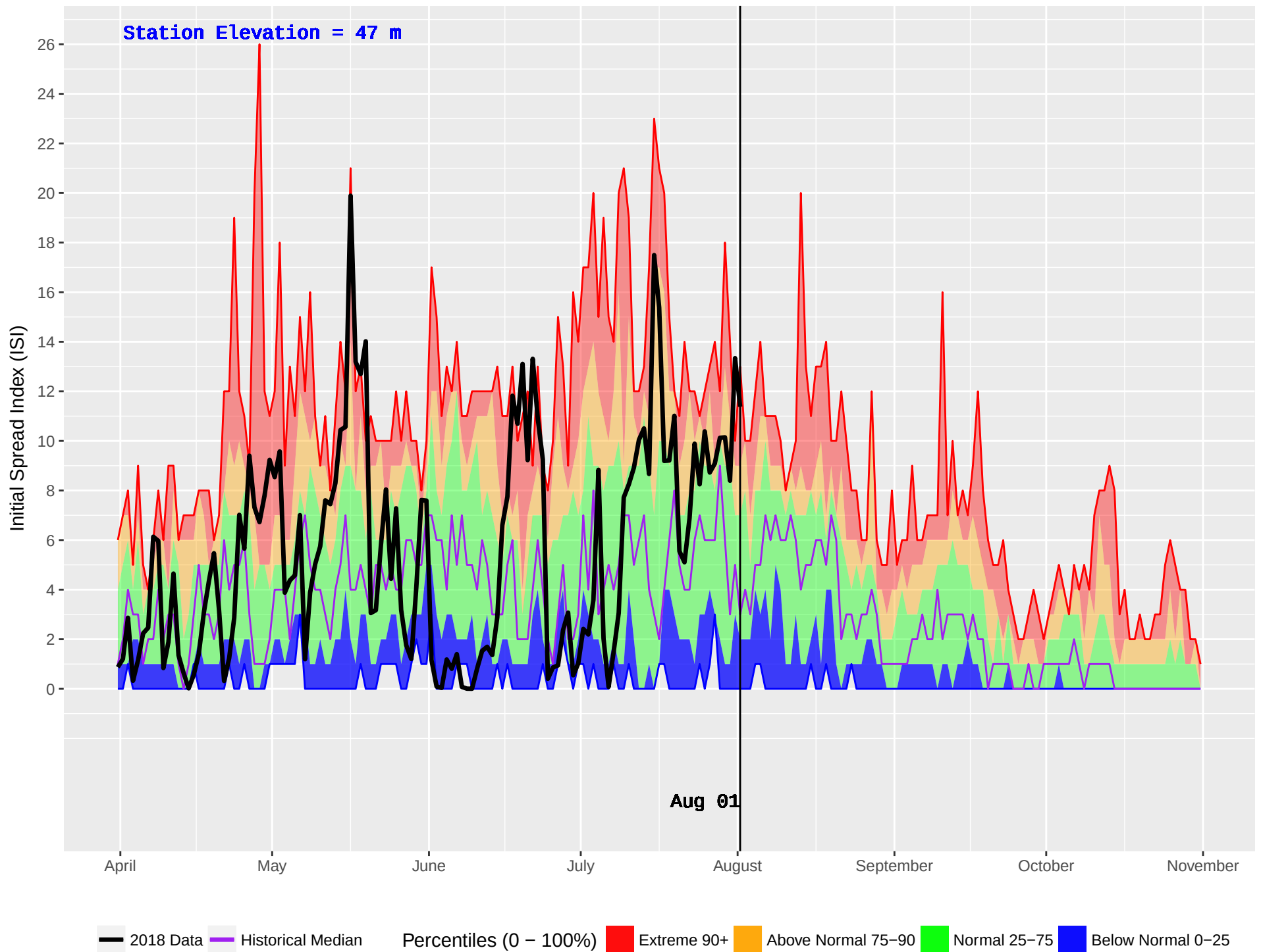
HAGENSBORG 2 (904) : Historical (2005–2016) and Current (2018) Daily Initial Spread Index (ISI)
