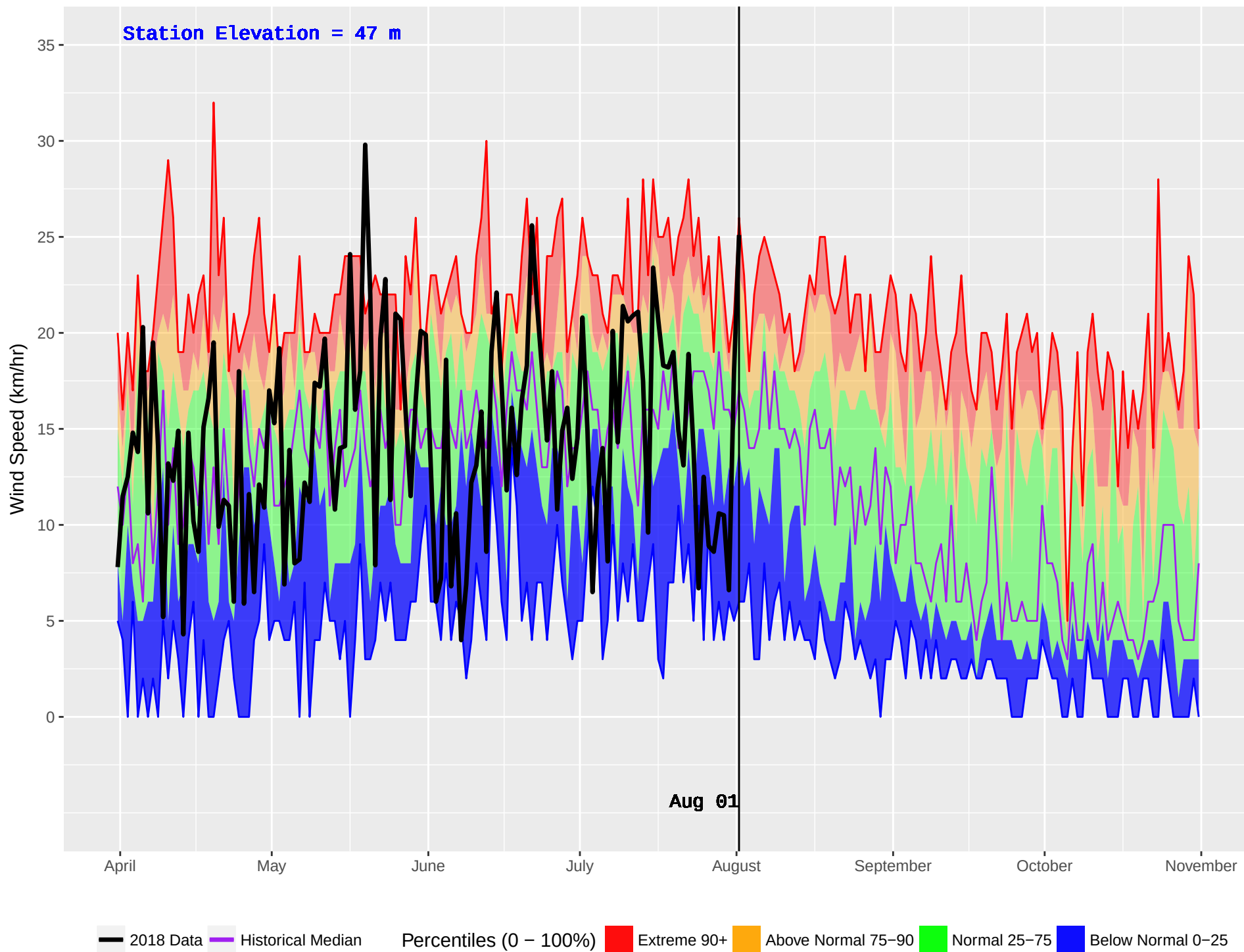
HAGENSBORG 2 (904) : Historical (2005–2016) and Current (2018) Daily Wind Speed
