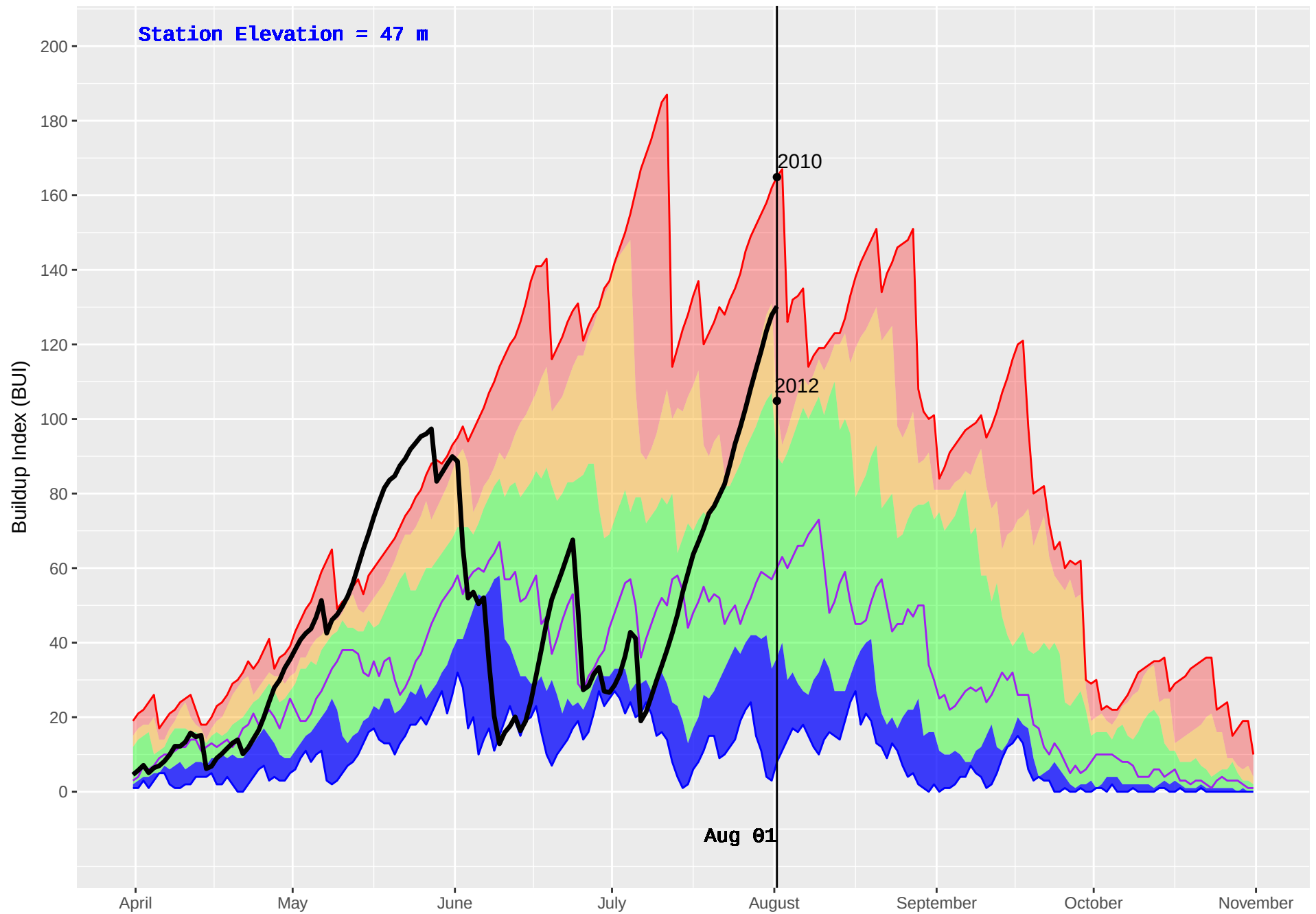
HAGENSBORG 2 (904) : Historical (2005–2016) and Current (2018) Daily Buildup Index (BUI)
