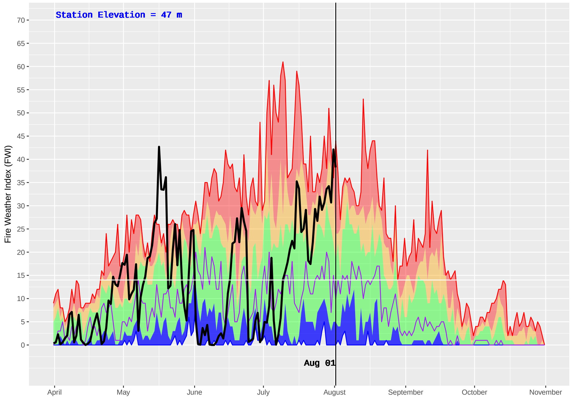
HAGENSBORG 2 (904) : Historical (2005–2016) and Current (2018) Daily Fire Weather Index (FWI)
