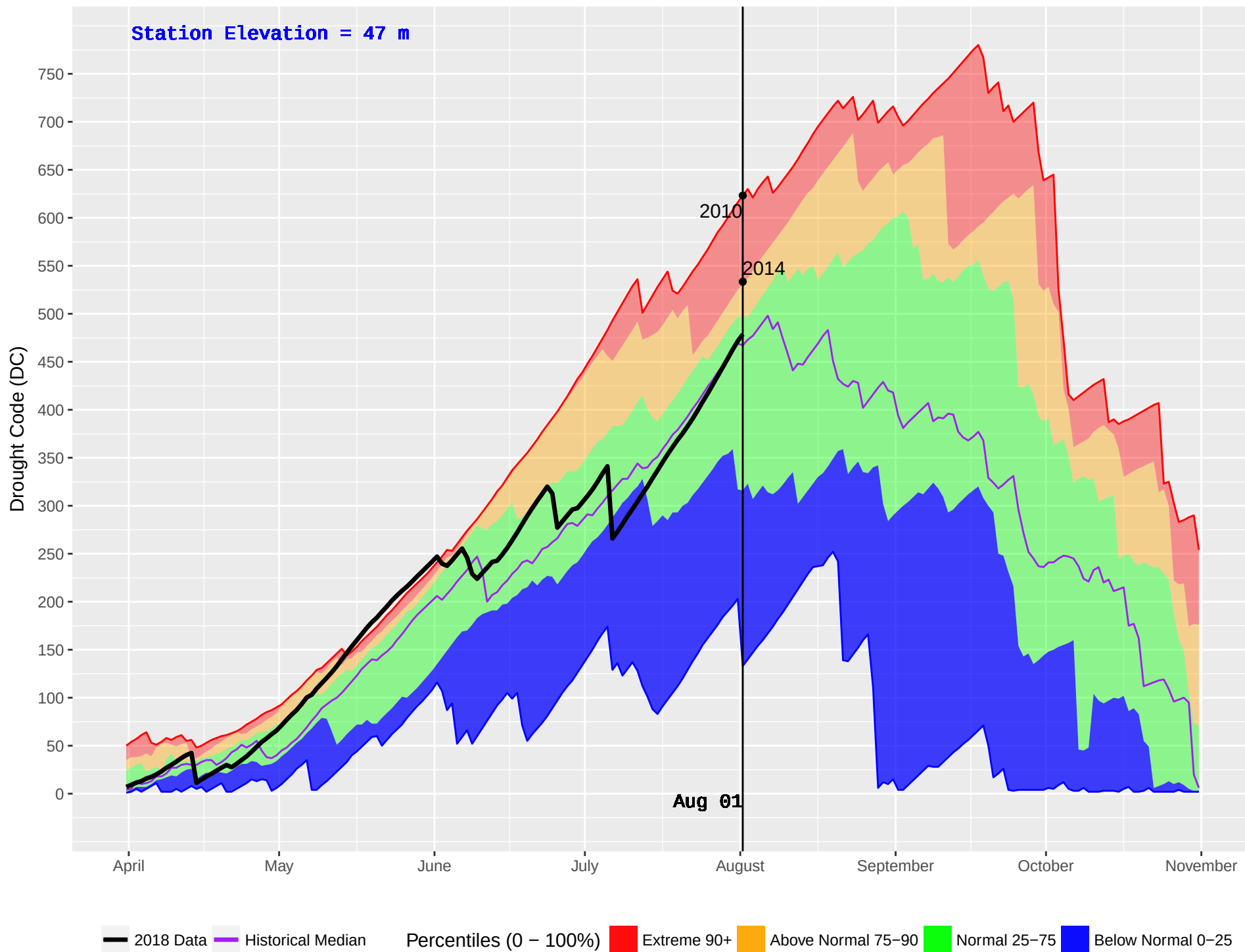
HAGENSBORG 2 (904) : Historical (2005–2016) and Current (2018) Daily Drought Code (DC)
